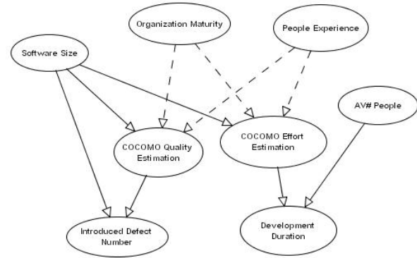
Figure 1. Component Estimation Model
