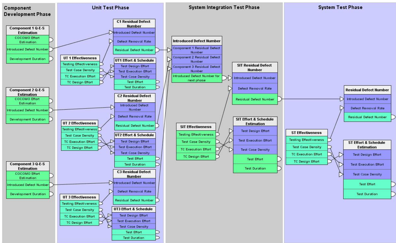
Figure 8. Project Level Estimation Model based on BBNs
