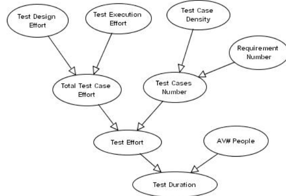
Figure 5. Test Estimation Model
